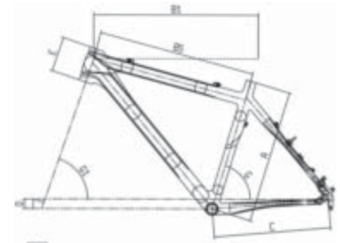
Geometry Racing Diletti Carbon Front Suspended
